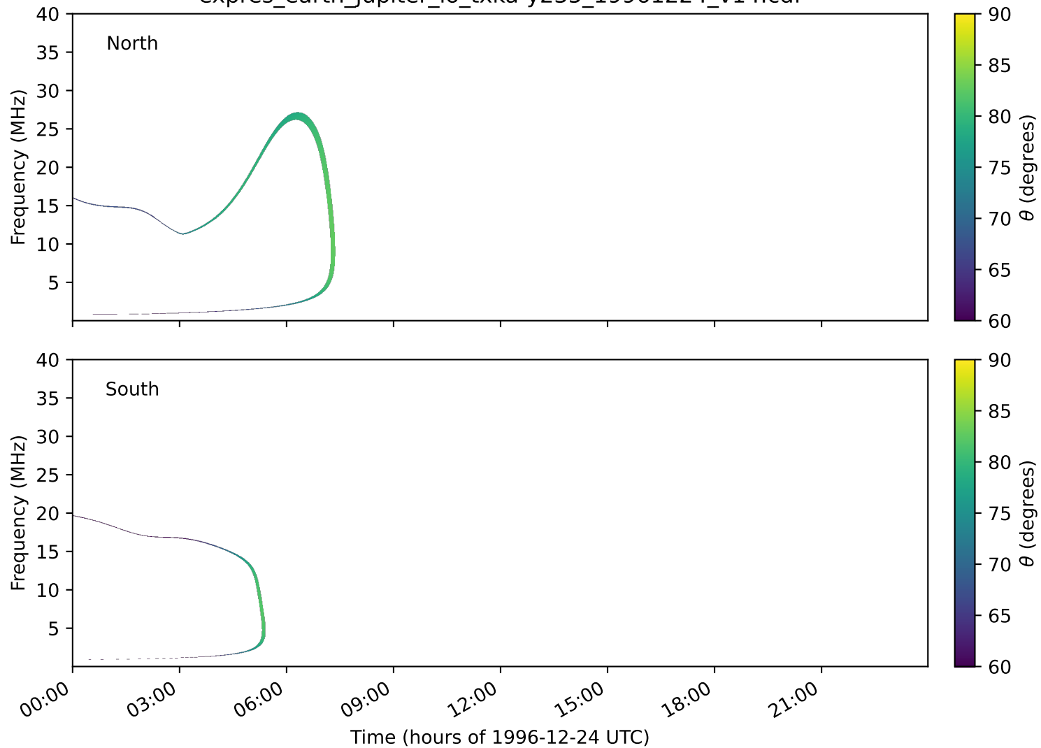
expres_earth_jupiter_io_txka-y235_19961224_v14.cdf
