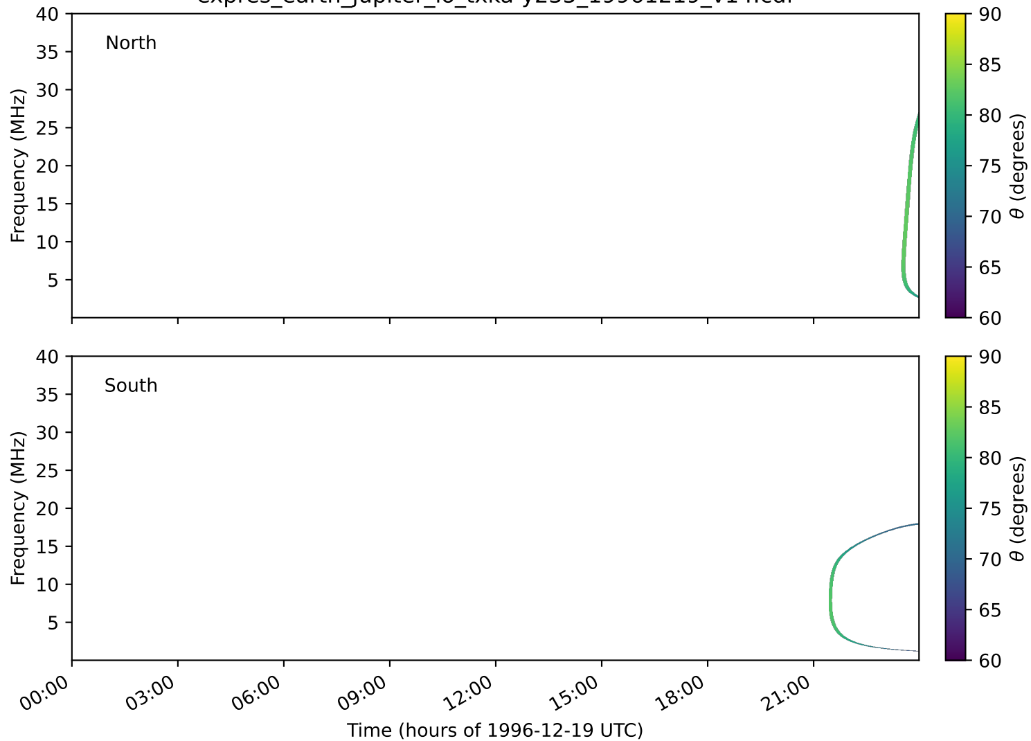
expres_earth_jupiter_io_txka-y235_19961219_v14.cdf
