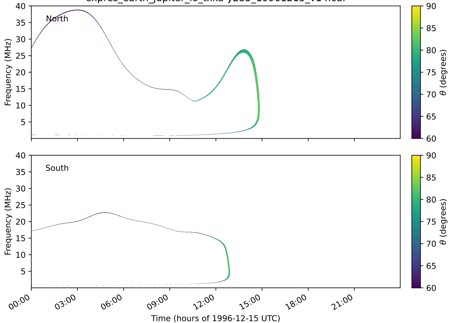
expres_earth_jupiter_io_txka-y235_19961215_v14.cdf
