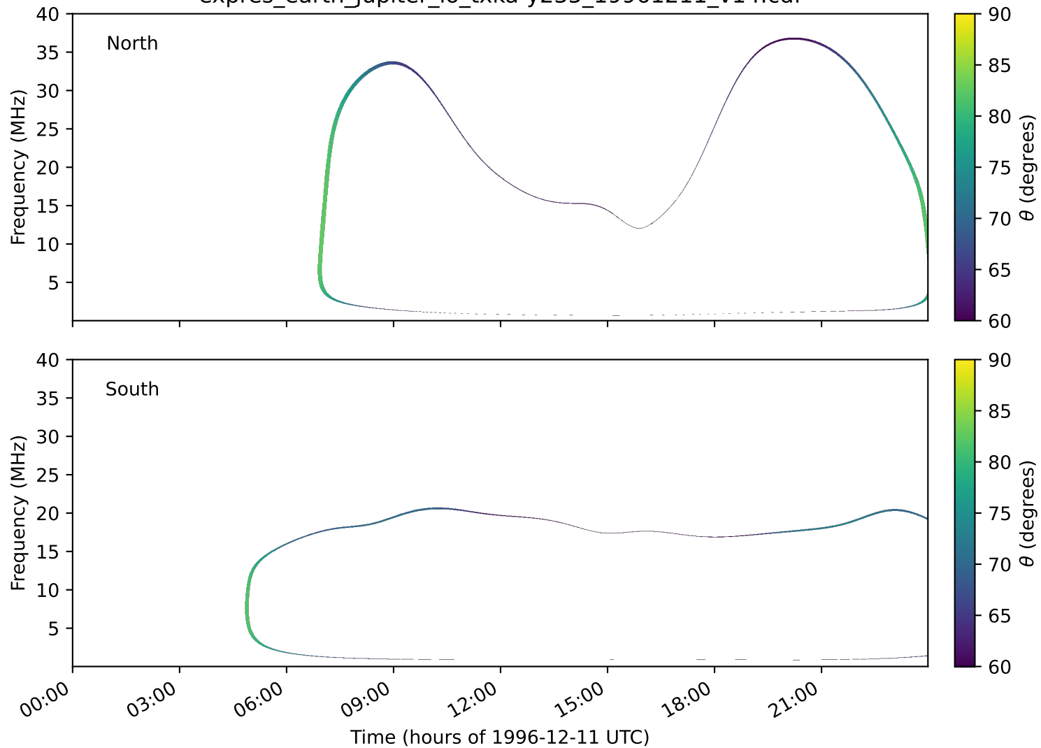
expres_earth_jupiter_io_txka-y235_19961211_v14.cdf
