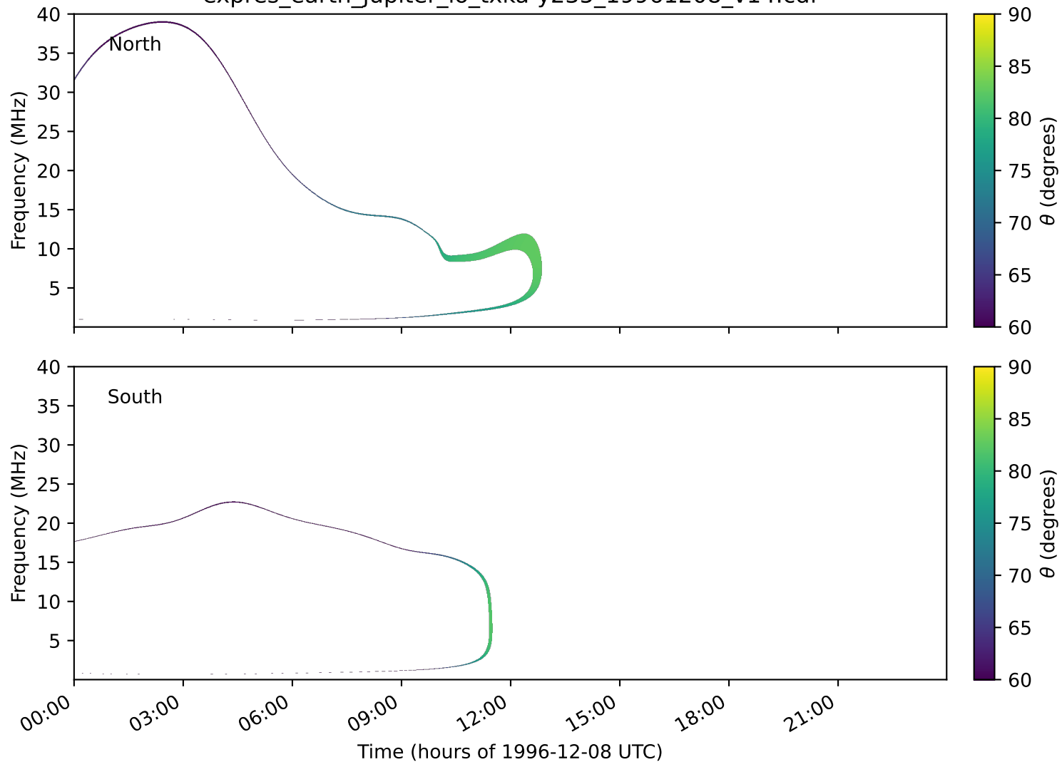
expres_earth_jupiter_io_txka-y235_19961208_v14.cdf
