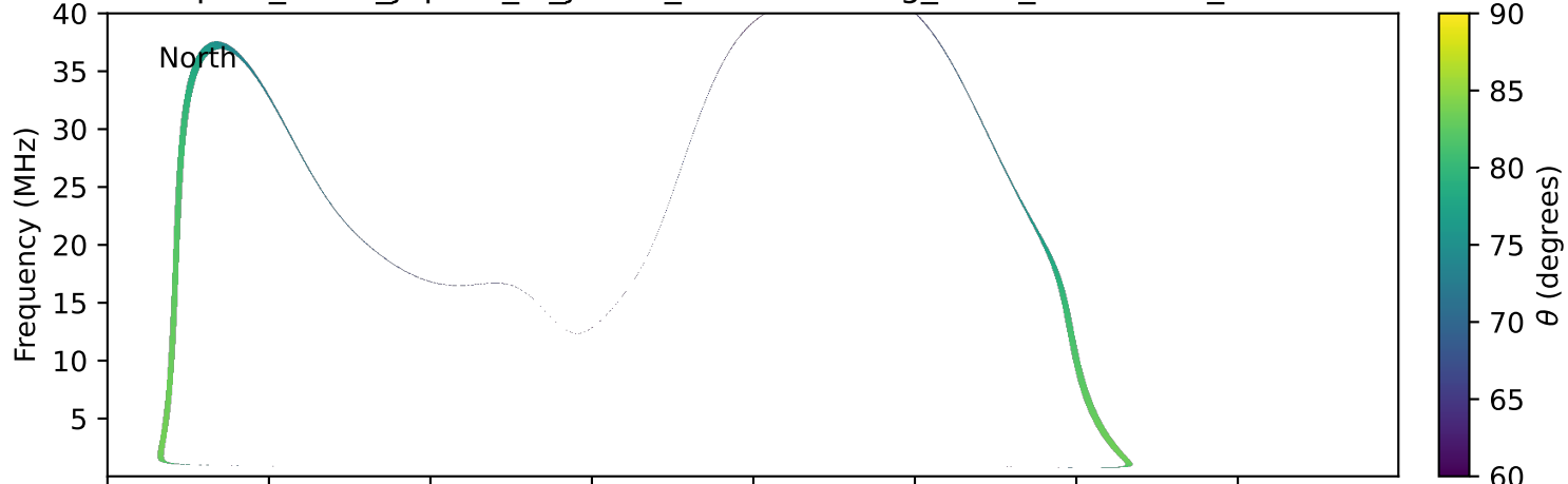
expres_earth_jupiter_io_jrm33_lossc-wid1deg_3kev_19961227_v11.cdf
