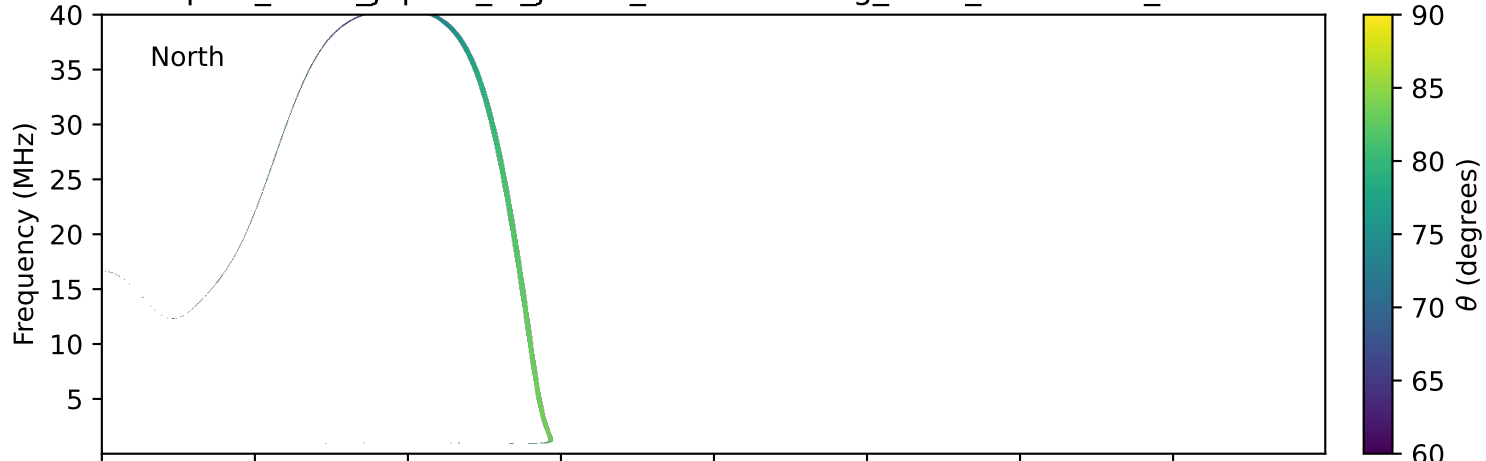
expres_earth_jupiter_io_jrm33_lossc-wid1deg_3kev_19961217_v11.cdf
