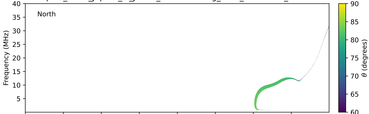
expres_earth_jupiter_io_jrm33_lossc-wid1deg_3kev_19961214_v11.cdf
