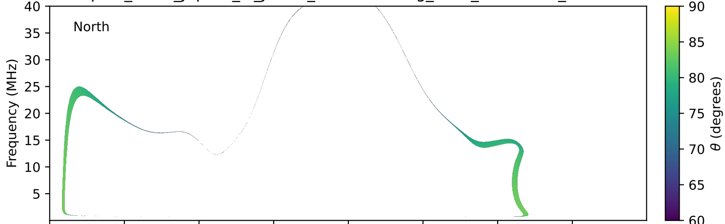
expres_earth_jupiter_io_jrm33_lossc-wid1deg_3kev_19961213_v11.cdf
