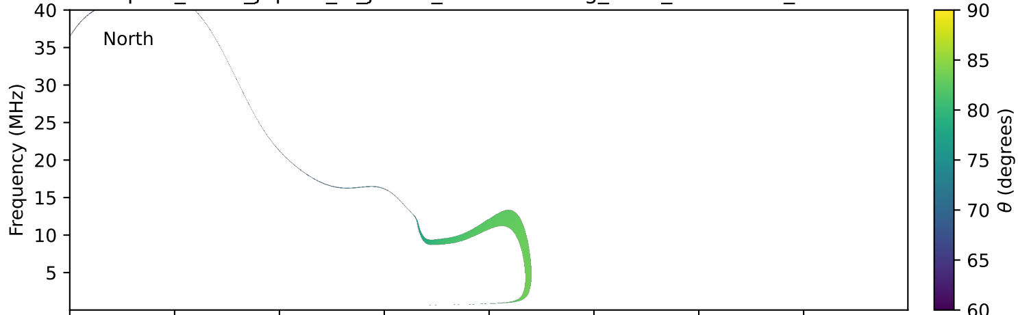
expres_earth_jupiter_io_jrm33_lossc-wid1deg_3kev_19961208_v11.cdf
