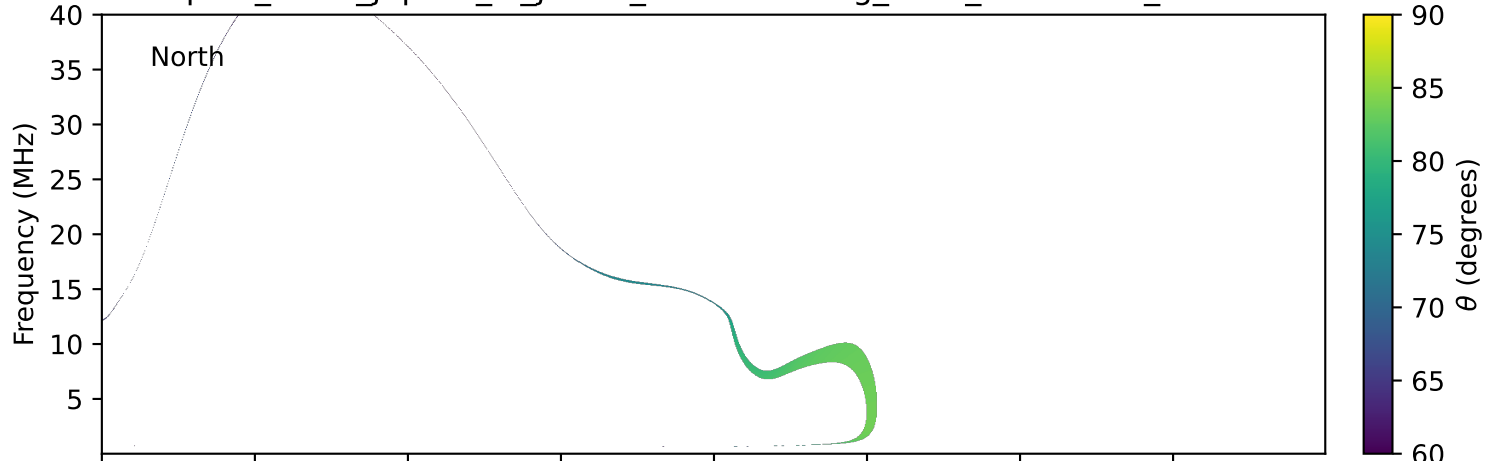
expres_earth_jupiter_io_jrm09_lossc-wid1deg_3kev_19961229_v11.cdf
