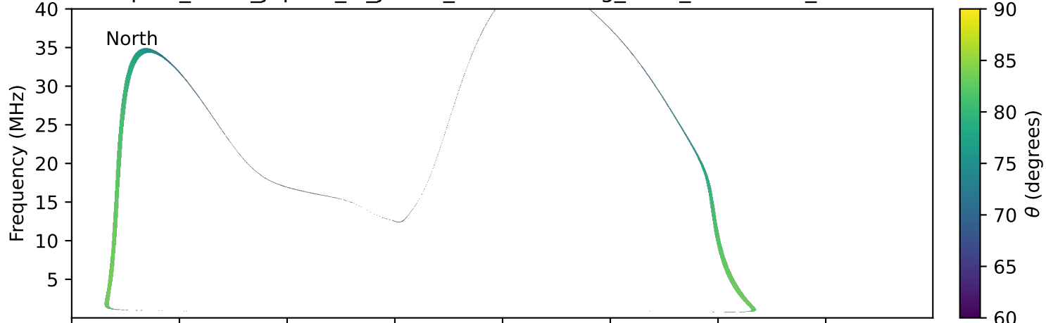
expres_earth_jupiter_io_jrm09_lossc-wid1deg_3kev_19961227_v11.cdf
