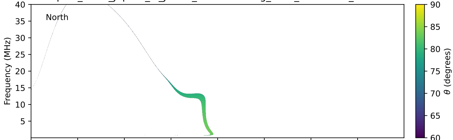
expres_earth_jupiter_io_jrm09_lossc-wid1deg_3kev_19961222_v11.cdf
