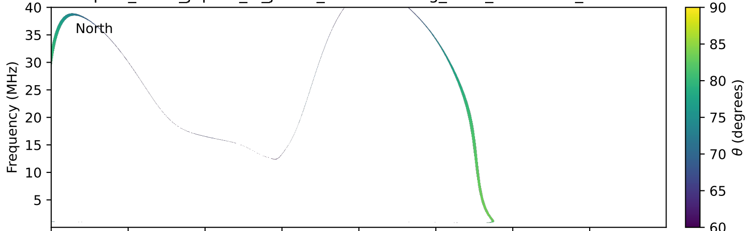
expres_earth_jupiter_io_jrm09_lossc-wid1deg_3kev_19961220_v11.cdf
