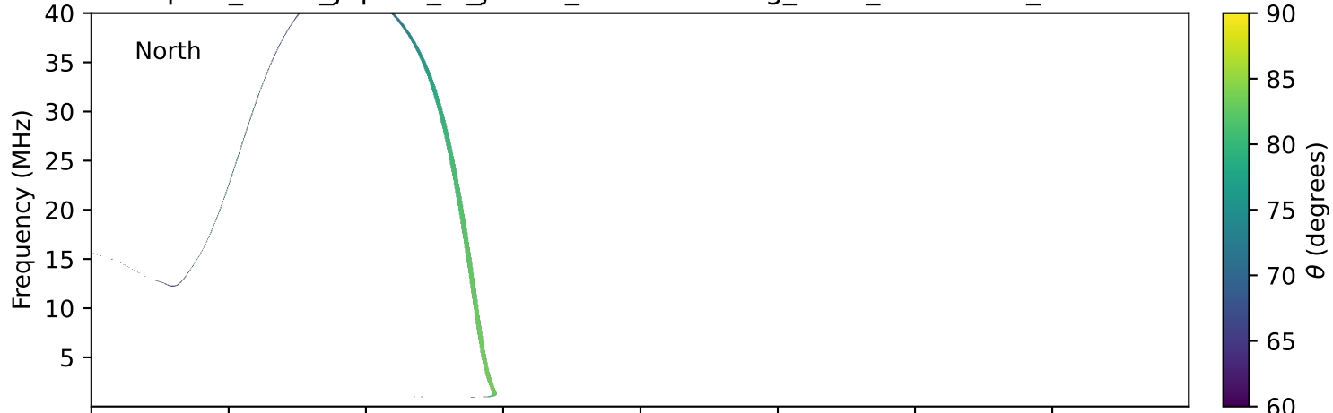
expres_earth_jupiter_io_jrm09_lossc-wid1deg_3kev_19961217_v11.cdf
