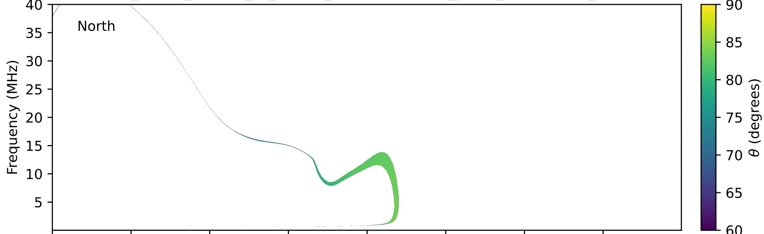
expres_earth_jupiter_io_jrm09_lossc-wid1deg_3kev_19961208_v11.cdf
