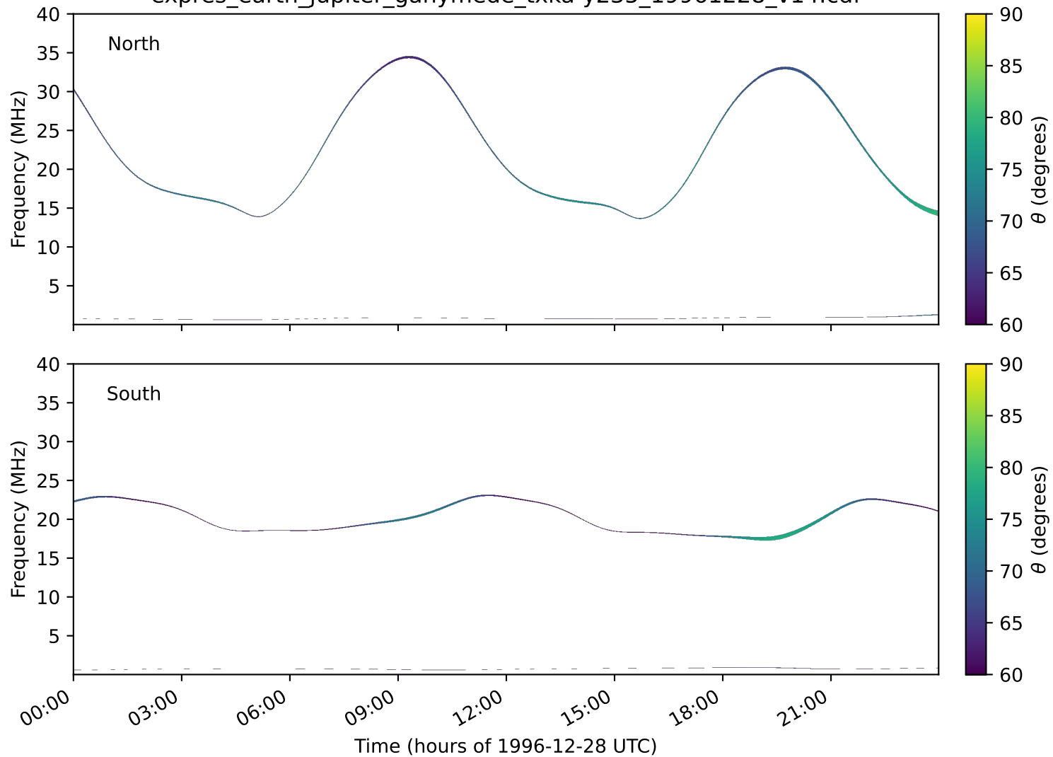
expres_earth_jupiter_ganymede_txka-y235_19961228_v14.cdf
