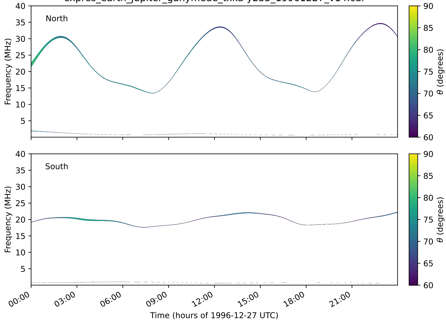
expres_earth_jupiter_ganymede_txka-y235_19961227_v14.cdf
