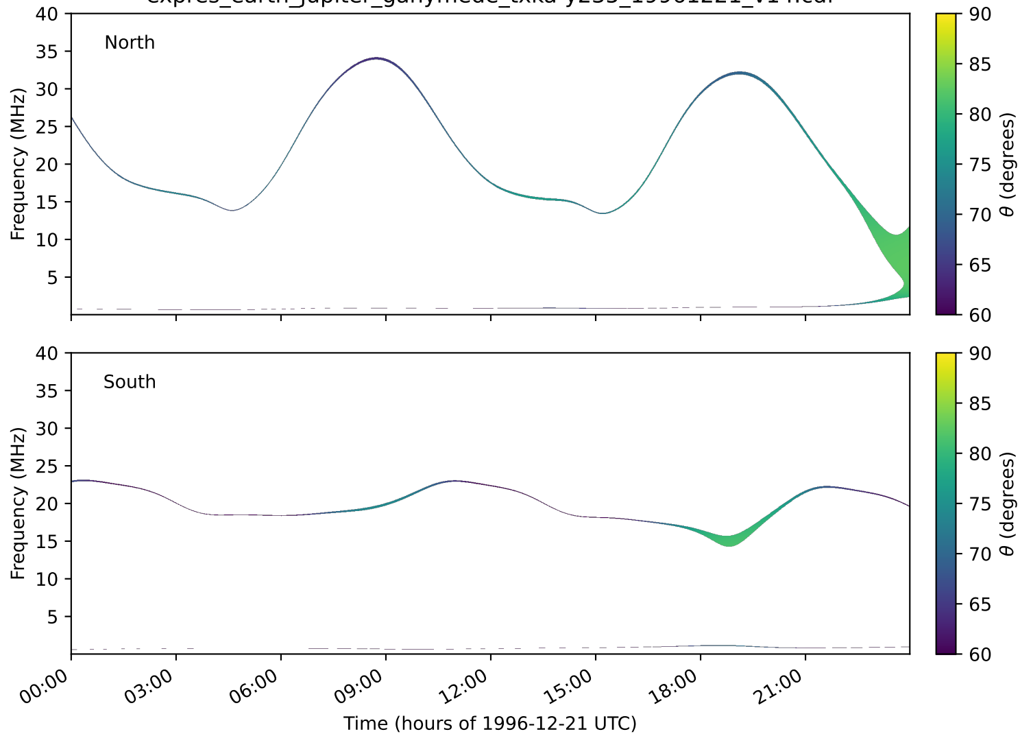
expres_earth_jupiter_ganymede_txka-y235_19961221_v14.cdf
