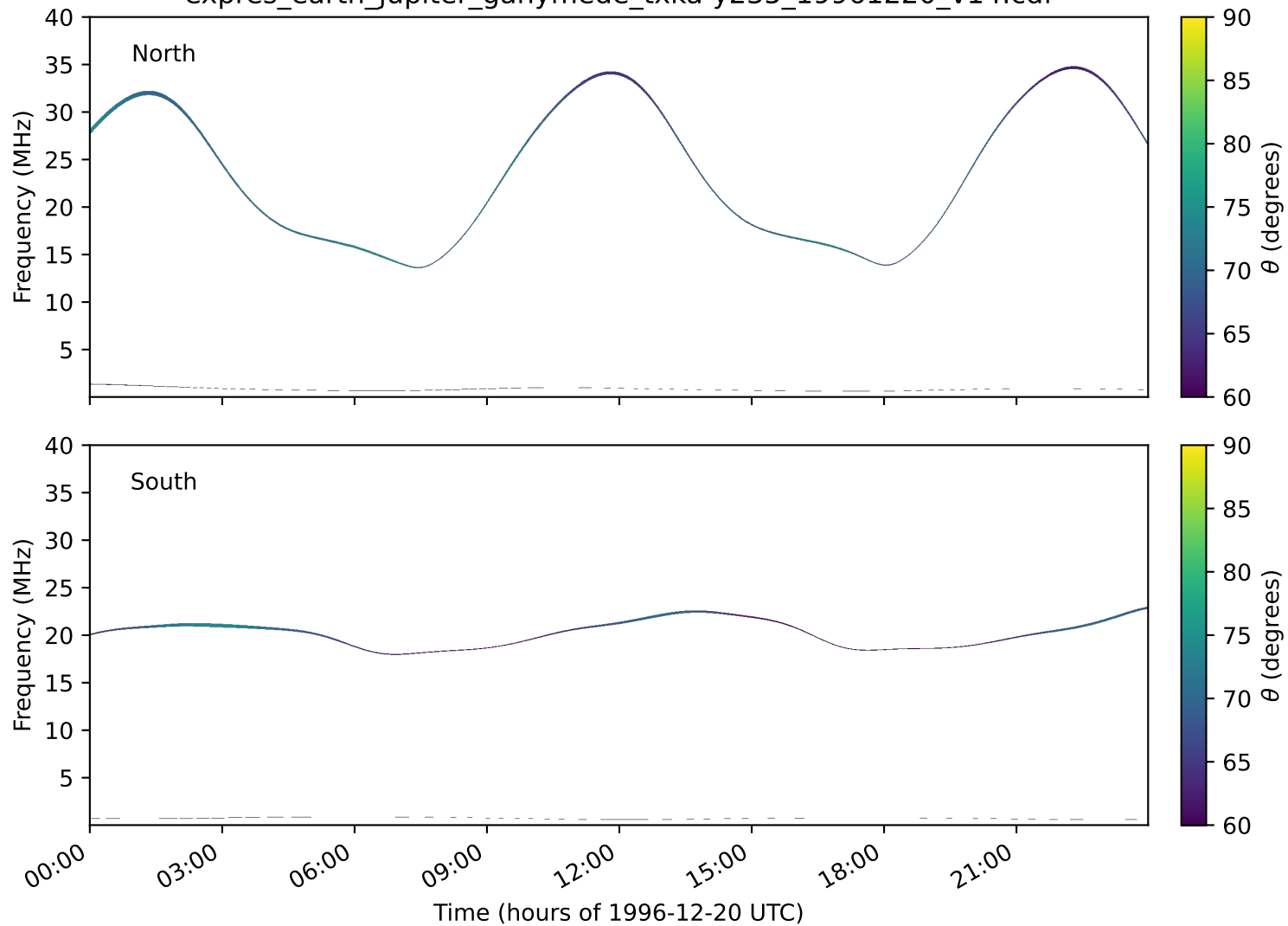
expres_earth_jupiter_ganymede_txka-y235_19961220_v14.cdf
