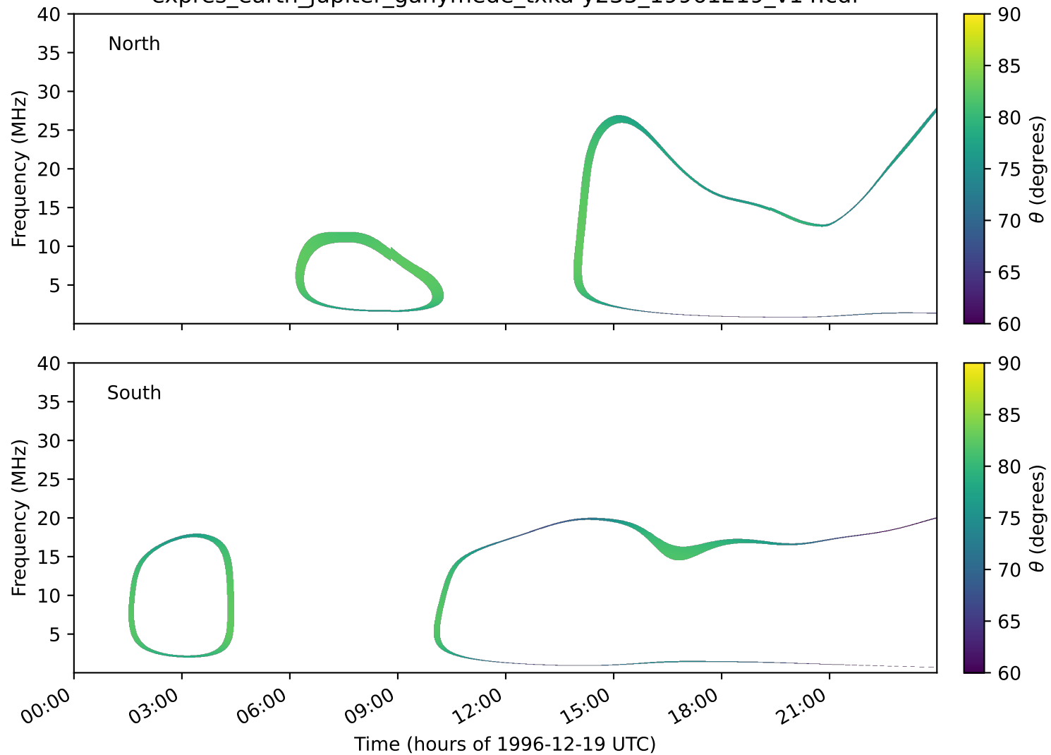
expres_earth_jupiter_ganymede_txka-y235_19961219_v14.cdf
