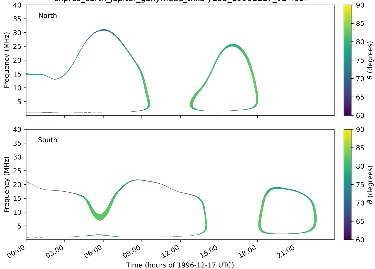
expres_earth_jupiter_ganymede_txka-y235_19961217_v14.cdf
