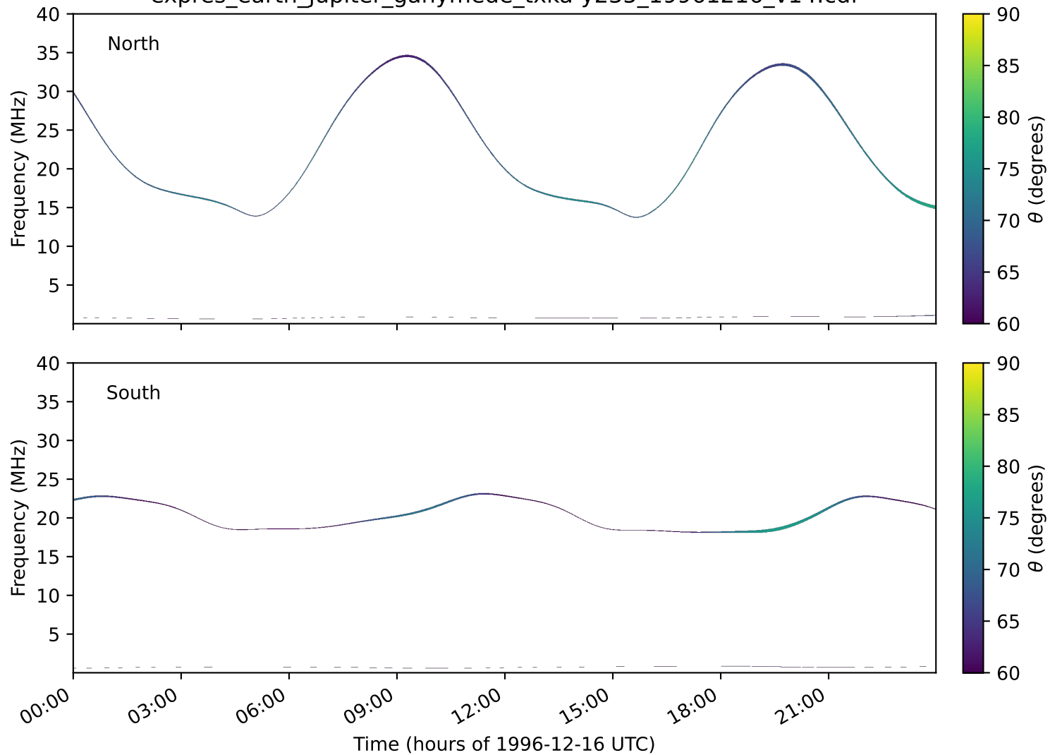
expres_earth_jupiter_ganymede_txka-y235_19961216_v14.cdf
