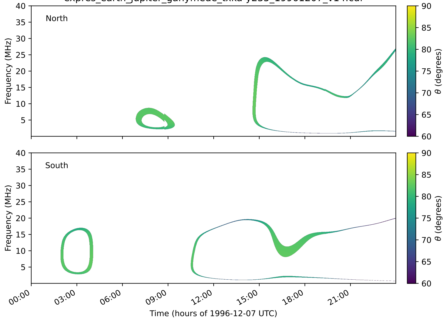
expres_earth_jupiter_ganymede_txka-y235_19961207_v14.cdf
