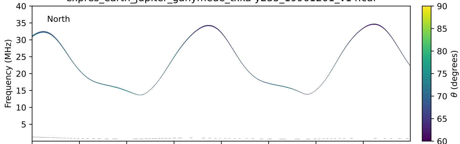
expres_earth_jupiter_ganymede_txka-y235_19961201_v14.cdf
