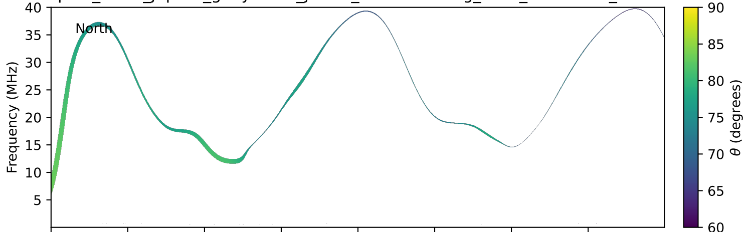
expres_earth_jupiter_ganymede_jrm33_lossc-wid1deg_3kev_19961227_v11.cdf
