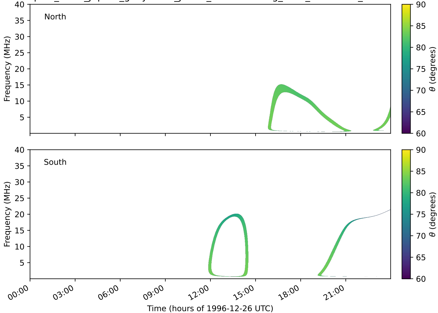
expres_earth_jupiter_ganymede_jrm33_lossc-wid1deg_3kev_19961226_v11.cdf
