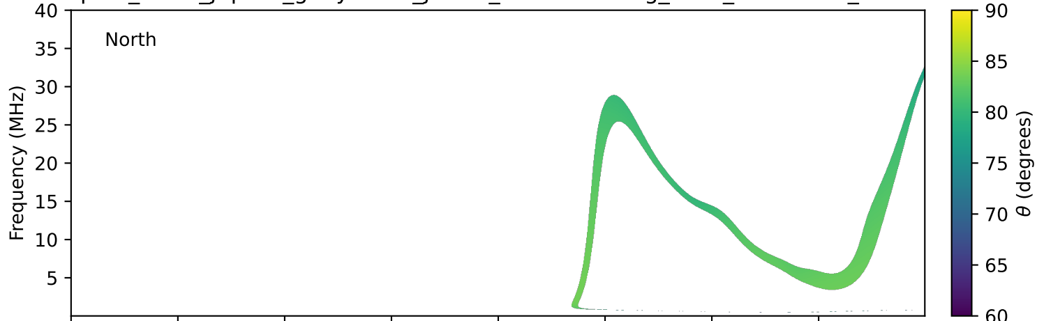
expres_earth_jupiter_ganymede_jrm33_lossc-wid1deg_3kev_19961219_v11.cdf
