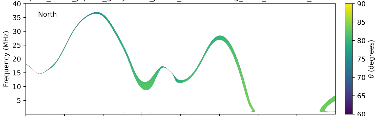
expres_earth_jupiter_ganymede_jrm33_lossc-wid1deg_3kev_19961210_v11.cdf
