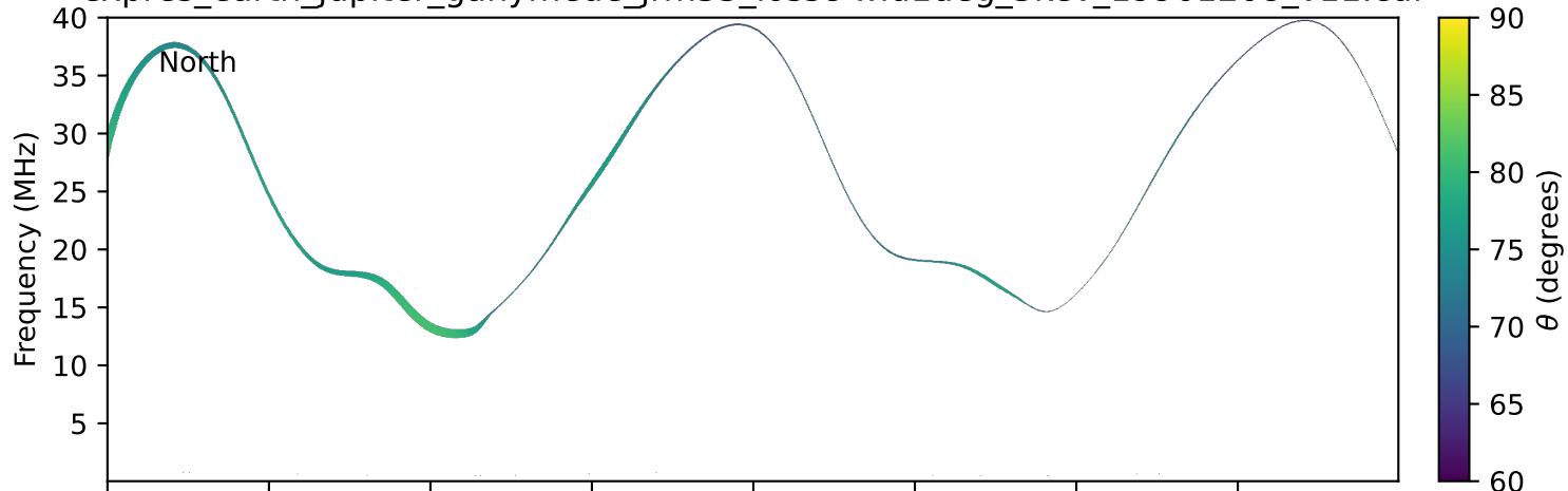
expres_earth_jupiter_ganymede_jrm33_lossc-wid1deg_3kev_19961208_v11.cdf
