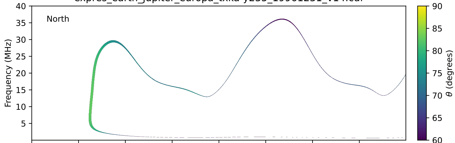
expres_earth_jupiter_europa_txka-y235_19961231_v14.cdf
