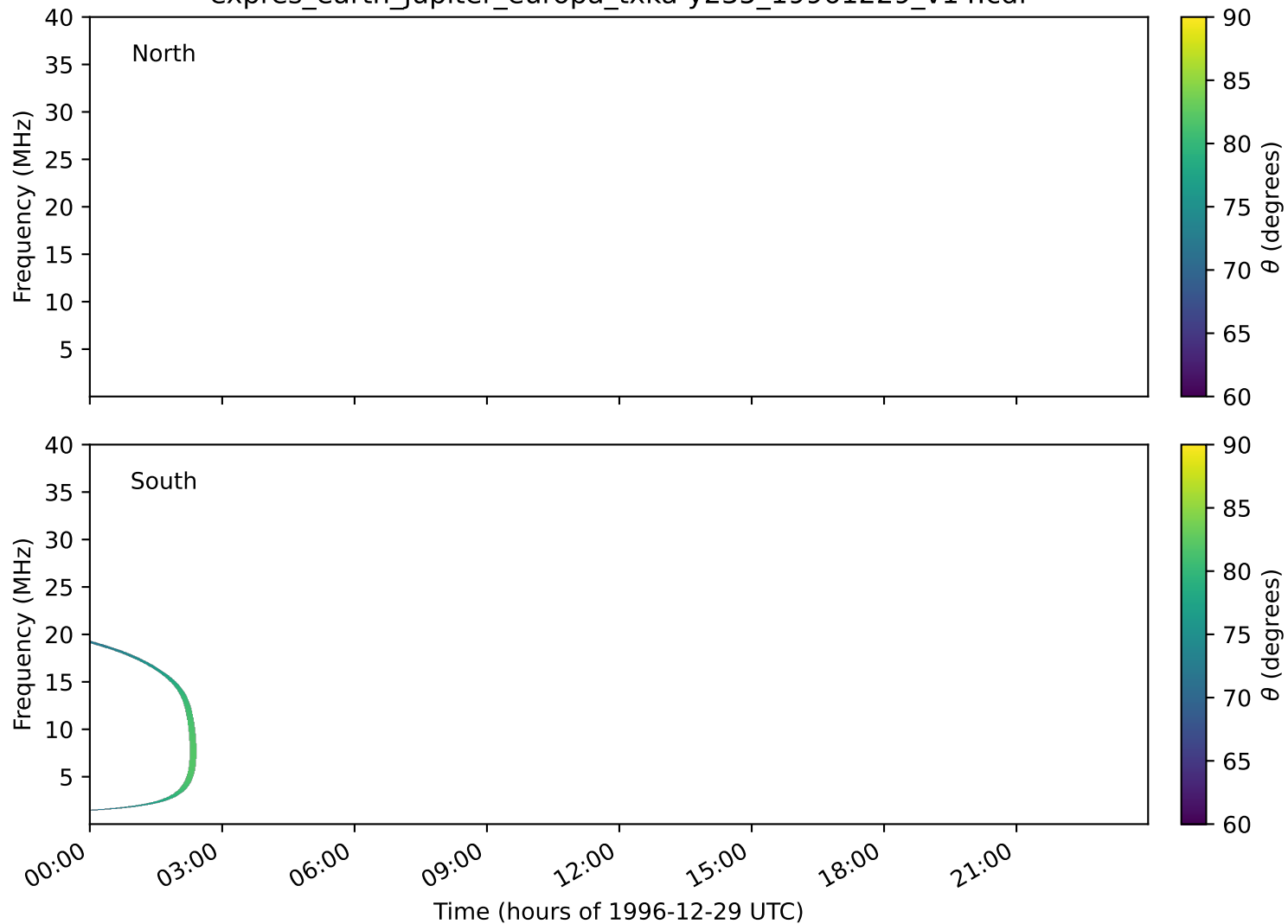
expres_earth_jupiter_europa_txka-y235_19961229_v14.cdf
