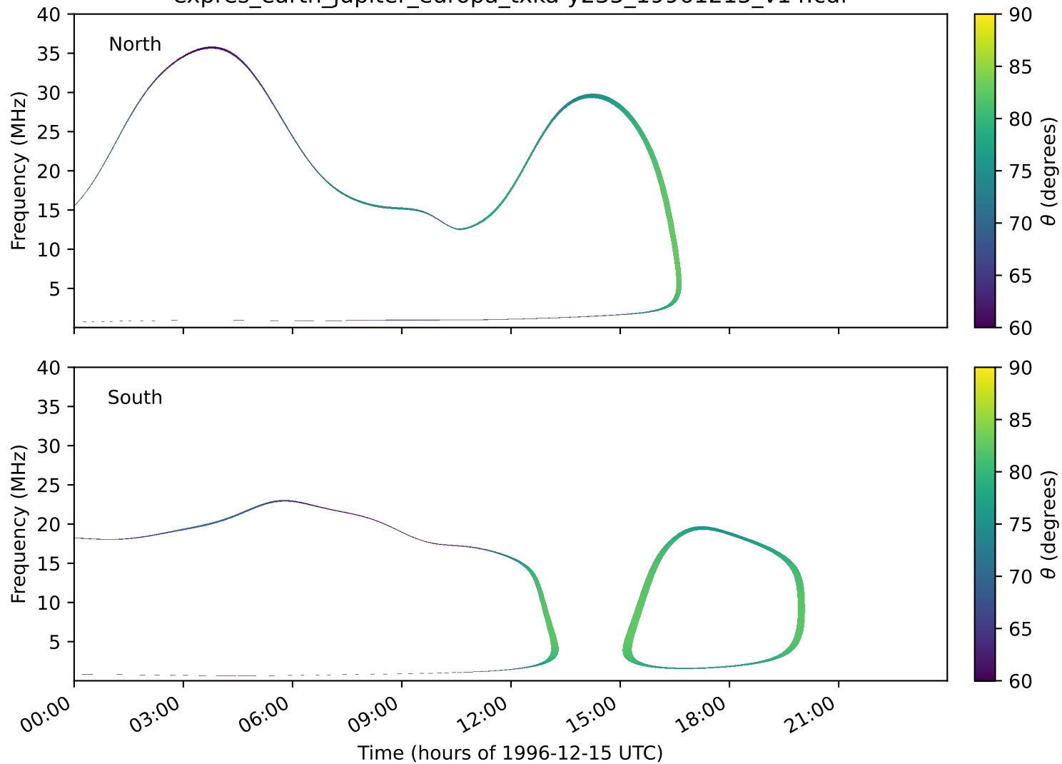
expres_earth_jupiter_europa_txka-y235_19961215_v14.cdf
