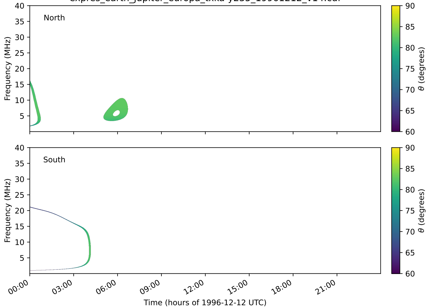
expres_earth_jupiter_europa_txka-y235_19961212_v14.cdf
