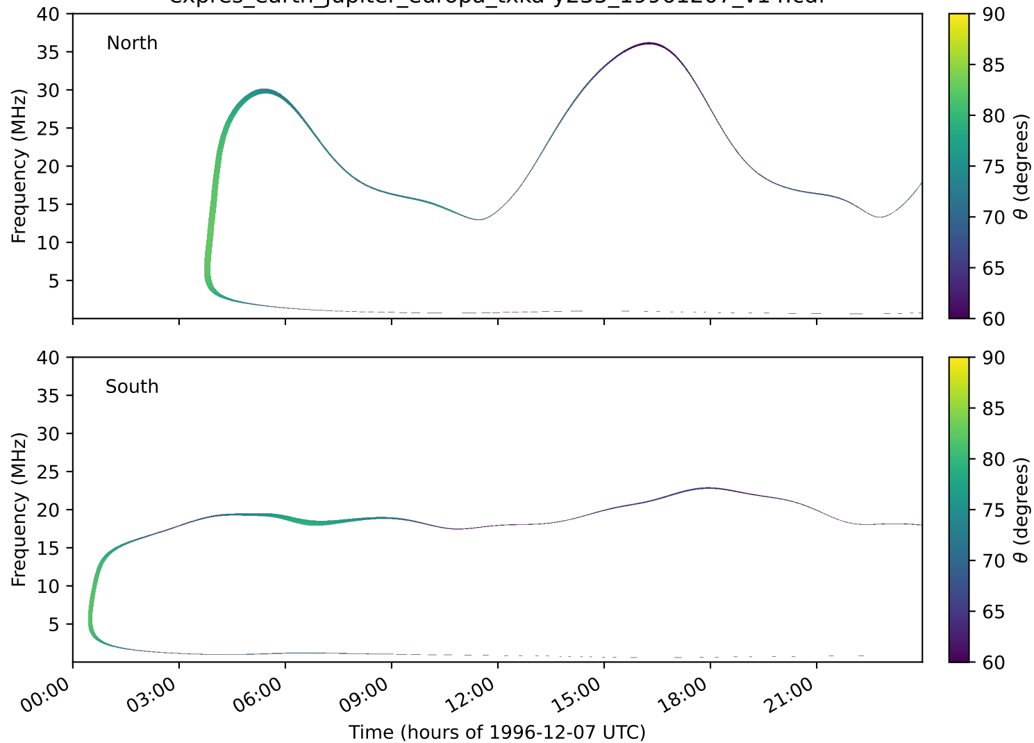
expres_earth_jupiter_europa_txka-y235_19961207_v14.cdf
