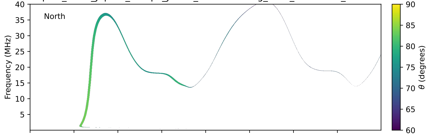
expres_earth_jupiter_europa_jrm33_lossc-wid1deg_3kev_19961231_v11.cdf
