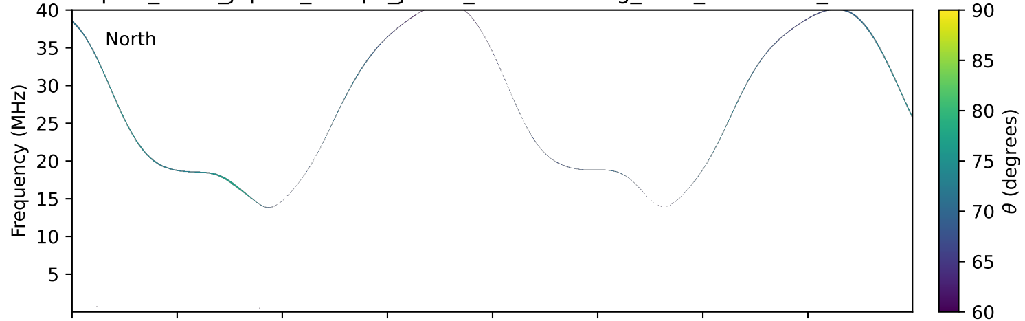
expres_earth_jupiter_europa_jrm33_lossc-wid1deg_3kev_19961218_v11.cdf
