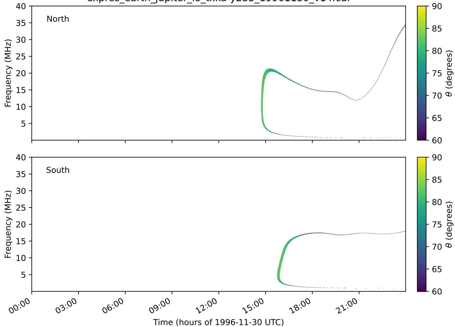
expres_earth_jupiter_io_txka-y235_19961130_v14.cdf
