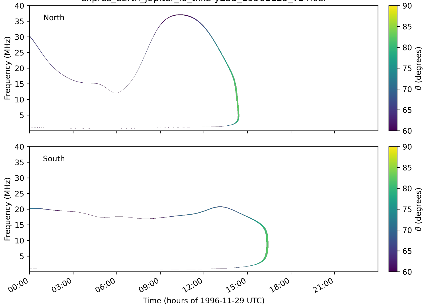
expres_earth_jupiter_io_txka-y235_19961129_v14.cdf
