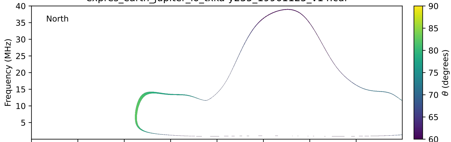
expres_earth_jupiter_io_txka-y235_19961125_v14.cdf
