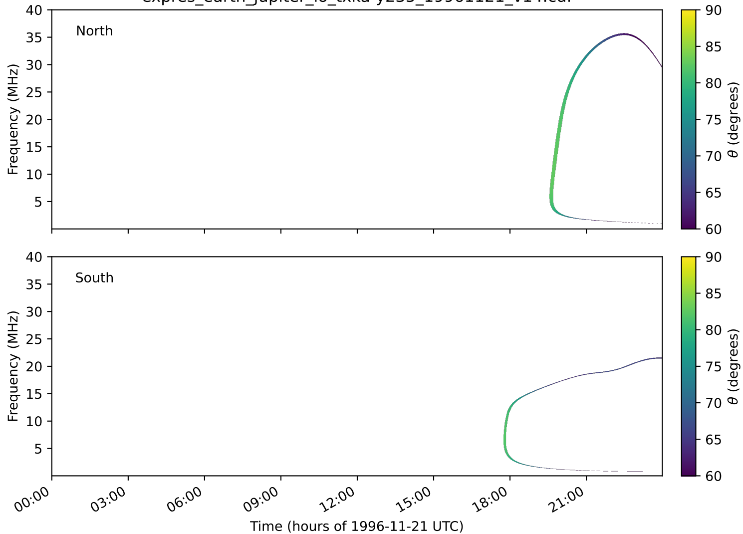
expres_earth_jupiter_io_txka-y235_19961121_v14.cdf
