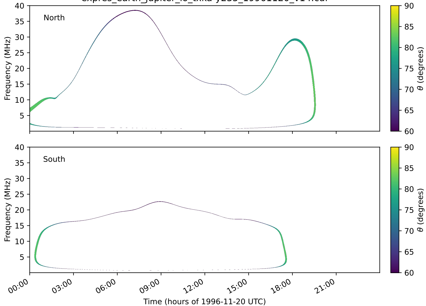
expres_earth_jupiter_io_txka-y235_19961120_v14.cdf
