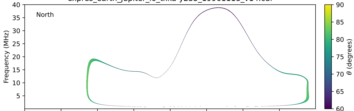
expres_earth_jupiter_io_txka-y235_19961118_v14.cdf
