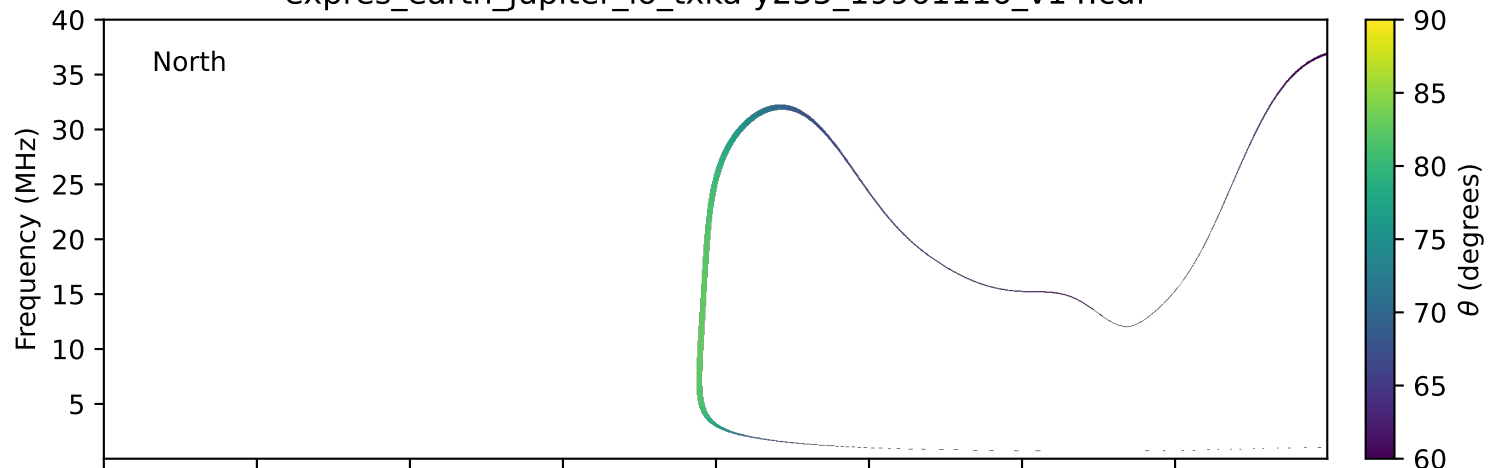
expres_earth_jupiter_io_txka-y235_19961116_v14.cdf
