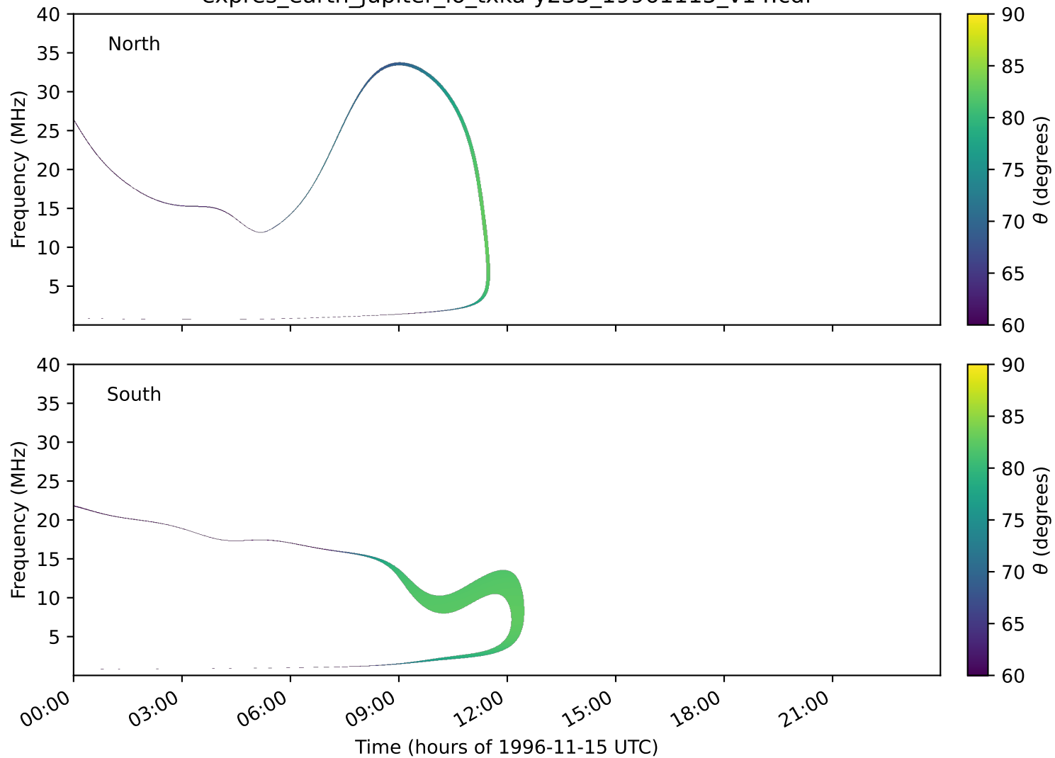
expres_earth_jupiter_io_txka-y235_19961115_v14.cdf
