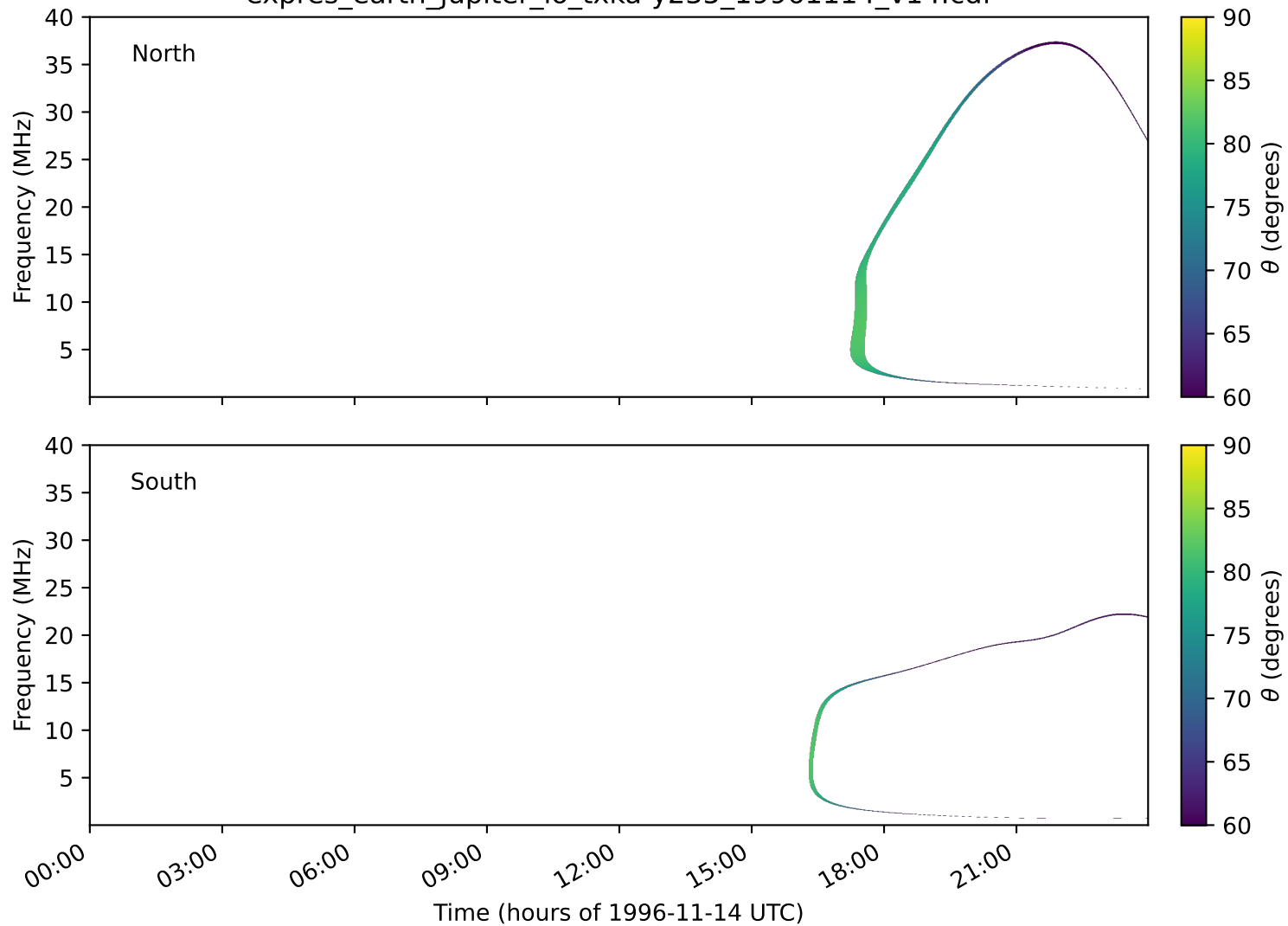
expres_earth_jupiter_io_txka-y235_19961114_v14.cdf
