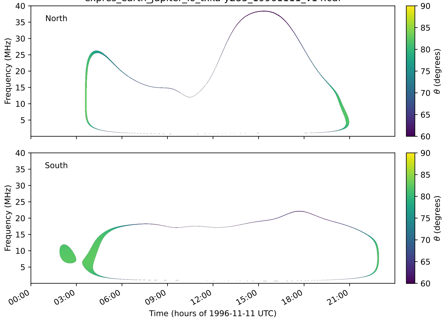
expres_earth_jupiter_io_txka-y235_19961111_v14.cdf
