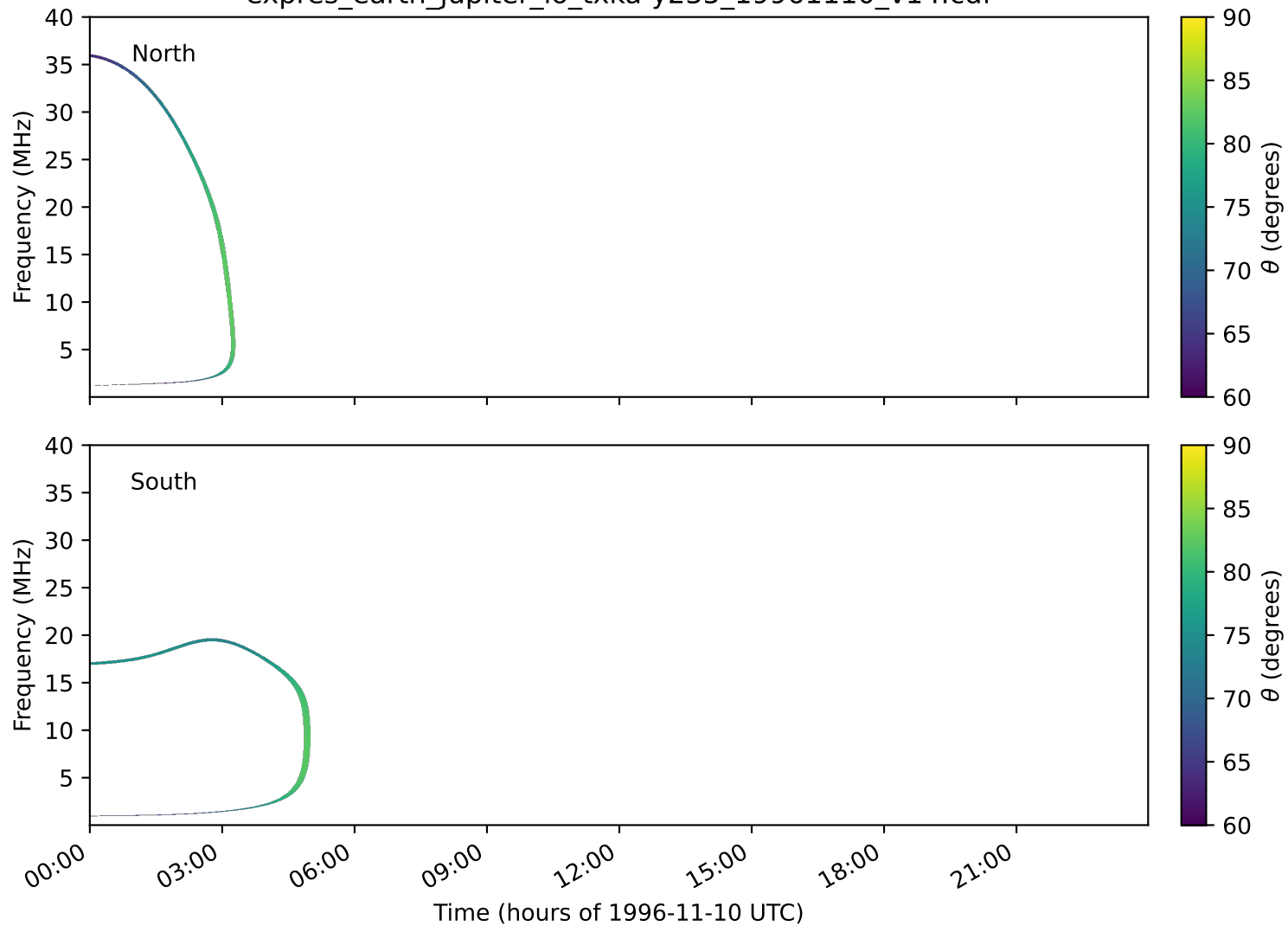
expres_earth_jupiter_io_txka-y235_19961110_v14.cdf
