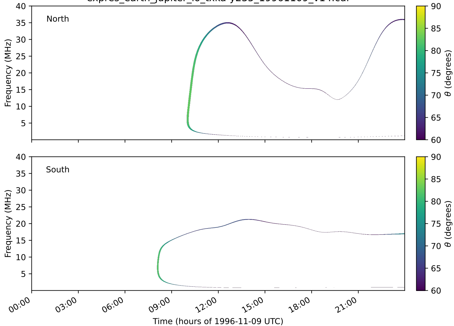
expres_earth_jupiter_io_txka-y235_19961109_v14.cdf
