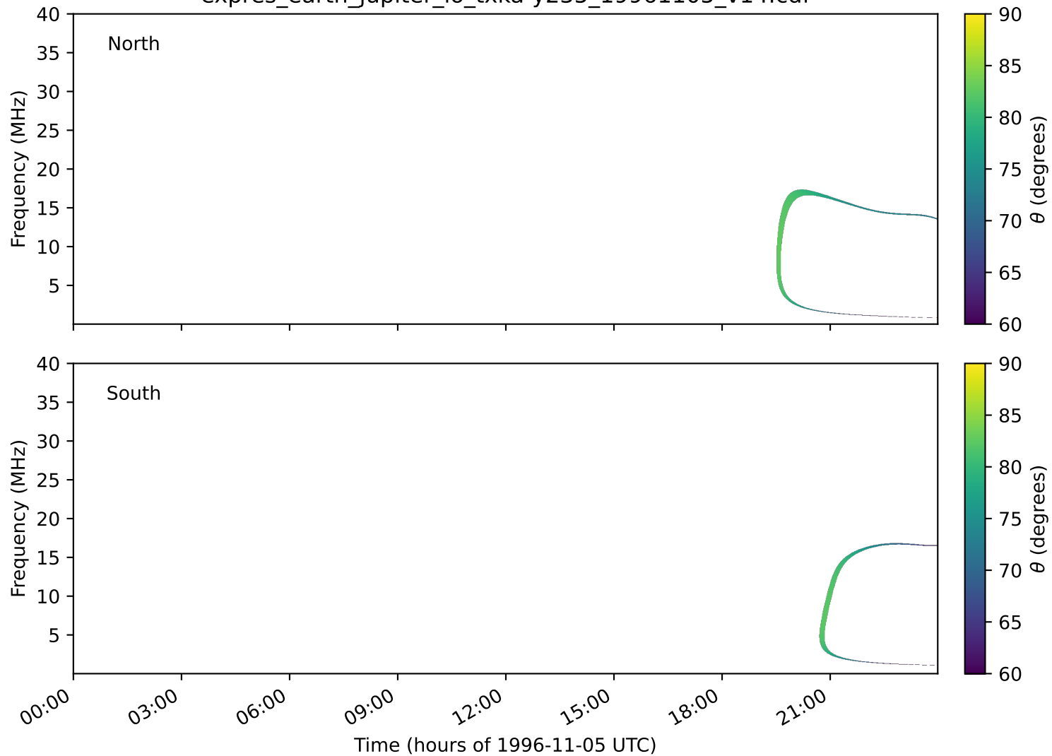
expres_earth_jupiter_io_txka-y235_19961105_v14.cdf
